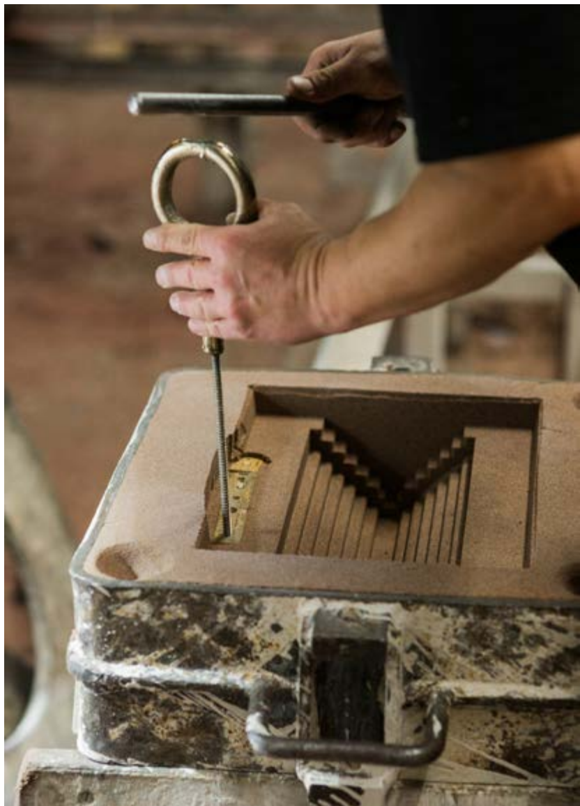
Sand mold for Tor casting
